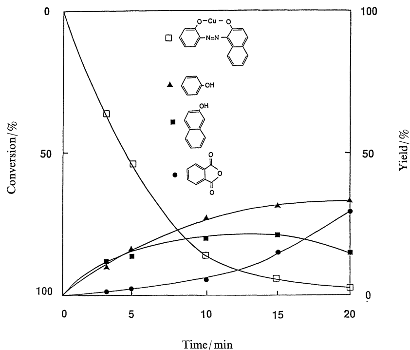
Fig. 4. Ozonization of 1-phenylazonaphthalene-2,2'-diolatocopper(II). Ozonization was carried out with an ozone-oxygen mixture ( O_3 : 0.068 mmol min -1 , O_2 : 200 ml min -1 ) on 1-phenylazonaphthalene-2,2'-diolatocopper(II) (1.6 mmol) in DMSO (2 ml) at 30 °C.
