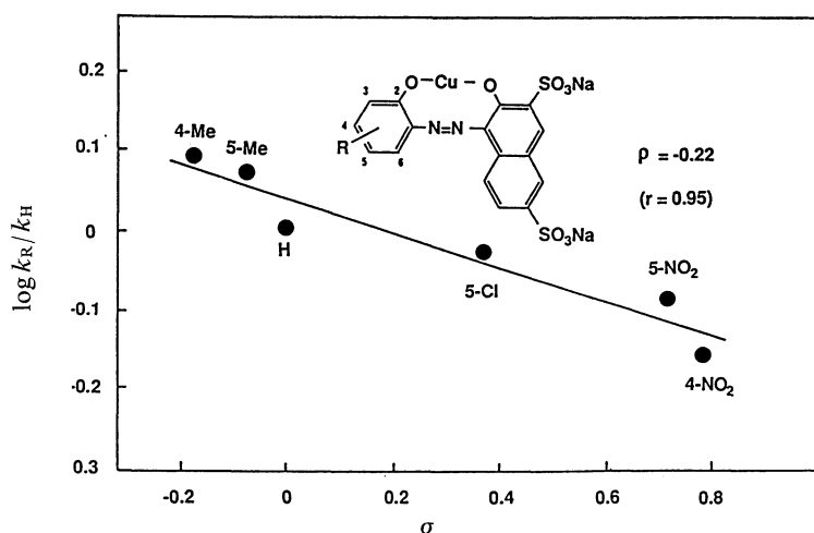
Fig. 3. Hammett's plots for the ozone fading of disodium 1-phenylazonaphthalene-3,6-disulfonate-2,2'-diolatocopper(II).
